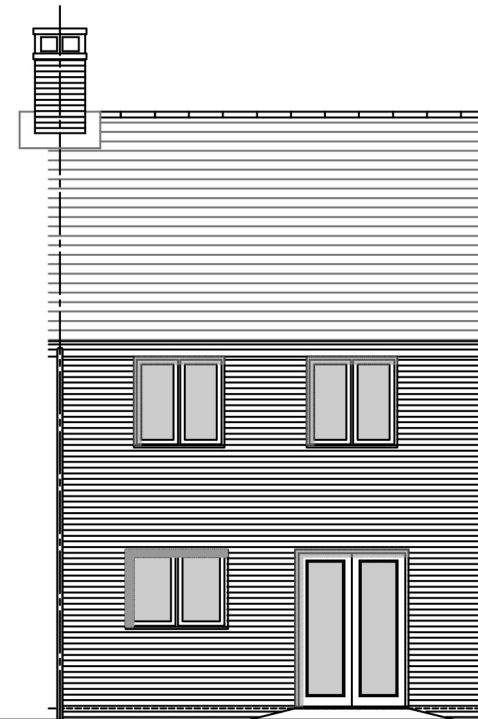
Rear Elevation
